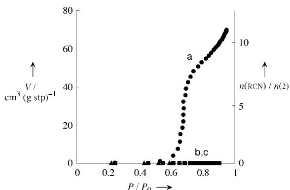
Figure 4. Sorption isotherm of nitriles at 298 K with 2 ( 0.1 \text{ g} , 2.85 \times 10^{-2} \text{ mmol} ): a) acetonitrile ( \bullet , P_0 = 10.7 \text{ kPa} ), b) propionitrile ( \blacksquare , P_0 = 6.27 \text{ kPa} ), and c) butyronitrile ( \blacktriangle , P_0 = 2.67 \text{ kPa} ).
